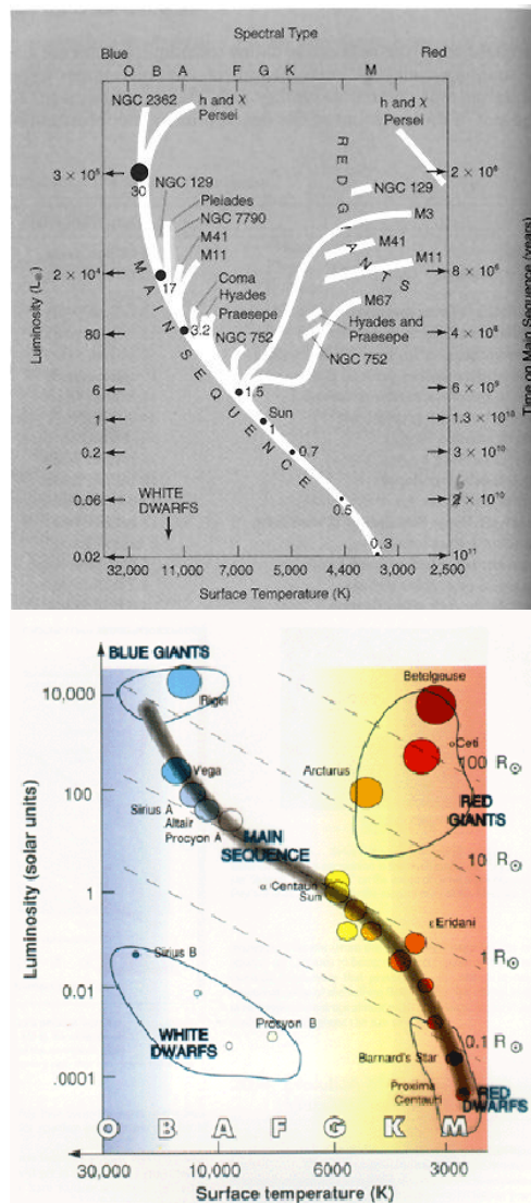
Figure 19 ,H-R Diagram
